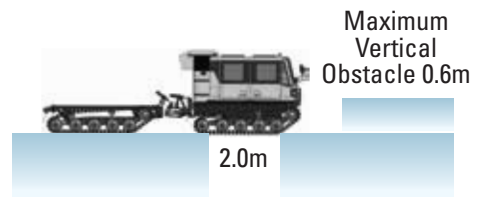
Trench Crossing
